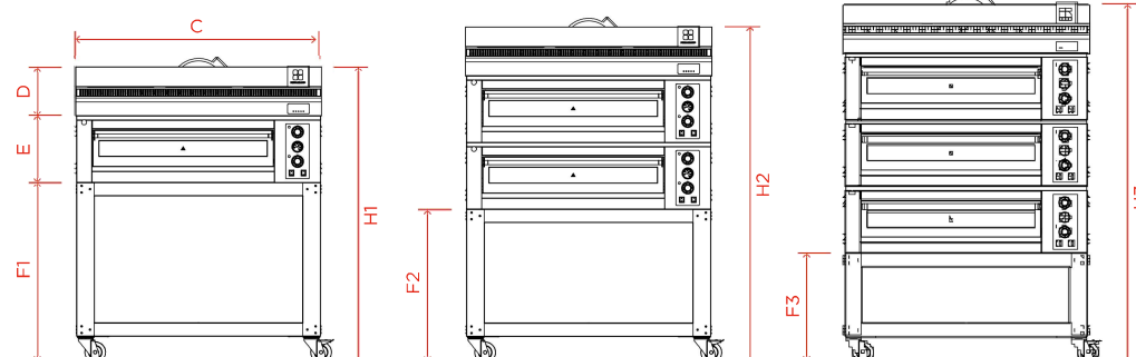
Front view / Pyralys HP 6L
