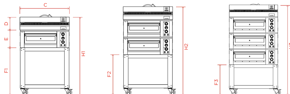
Front view / Pyralys HP 4
